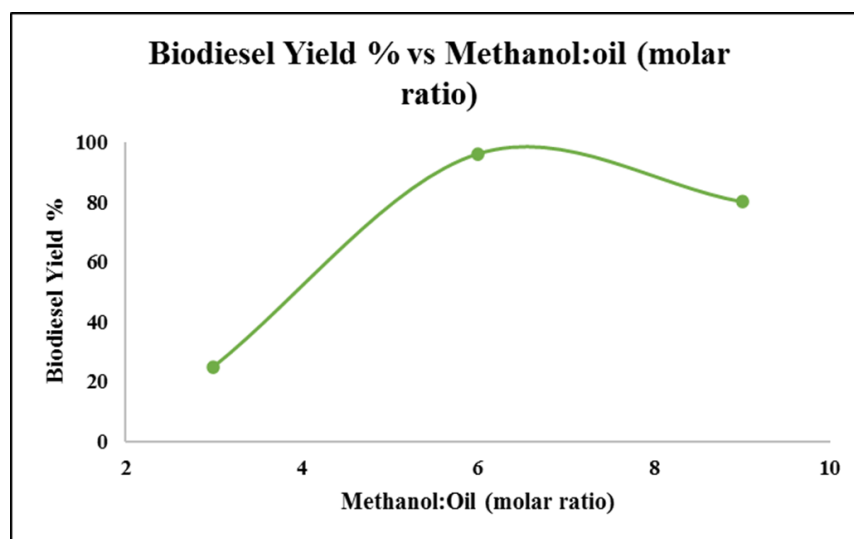
Figure 3. Effect of molar ratio on ML biodiesel yield.
