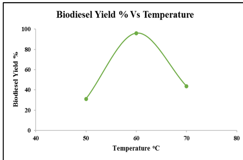
Figure 4. Effect of temperature on ML Biodiesel yield.
