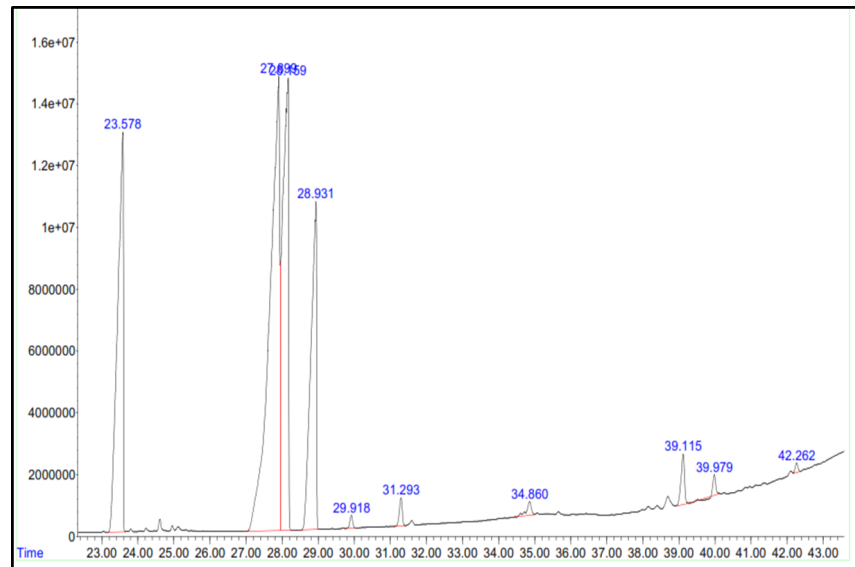
Figure 6. GC-FID chromatogram of the biodiesel produced from Mahua oil.
