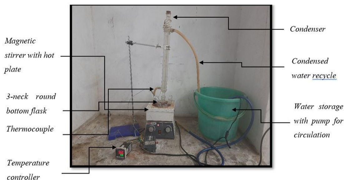
Figure 1. Biodiesel batch reactor.
