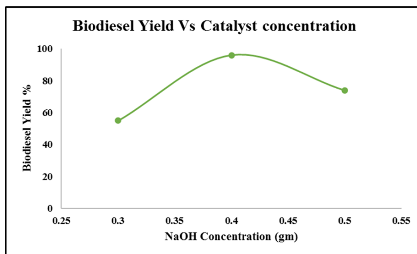
Figure 2. Effect catalyst concentration on biodiesel yield.
